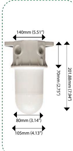
ROOF MOUNT JUNCTION BOX
